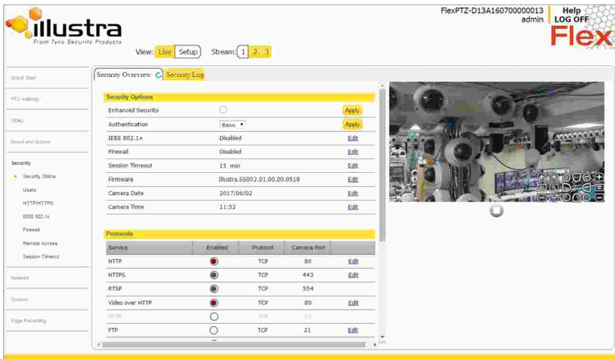
Figure 7-1 Security Menu
