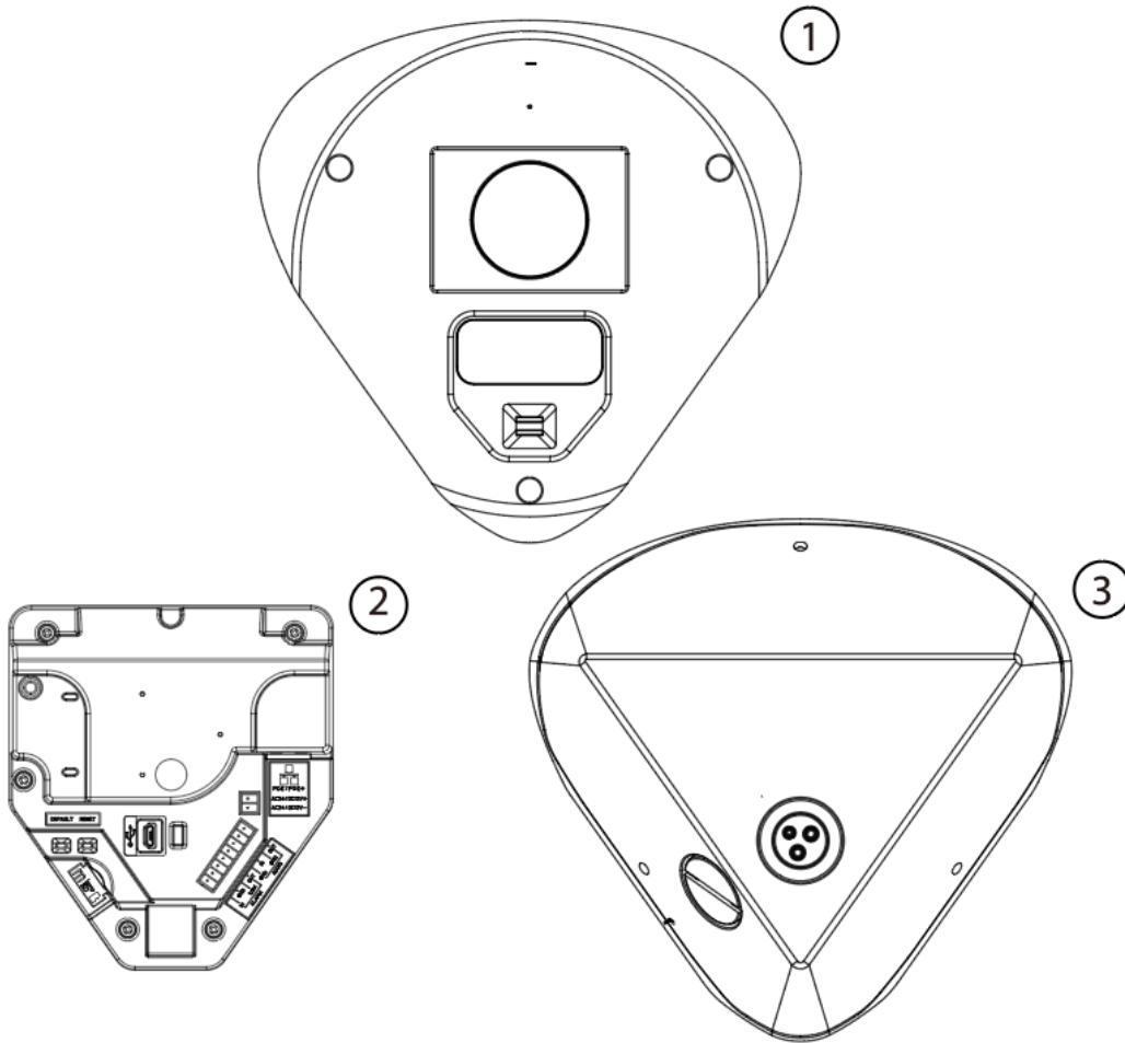
Figure 36 Camera parts
