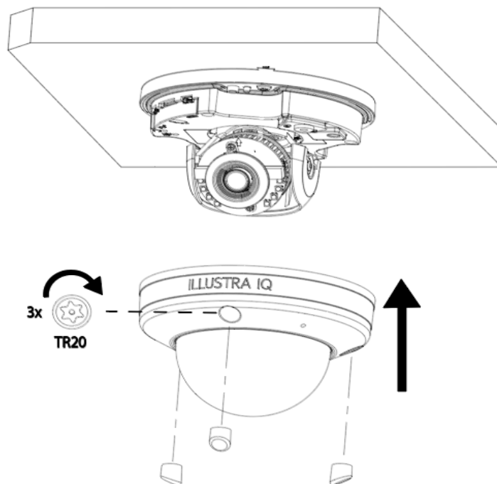
Figure 52 Installing the camera onto a wall or ceiling (continued)
