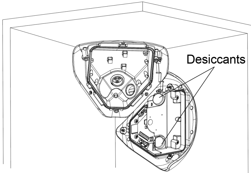
Figure 45 Desiccant bags
