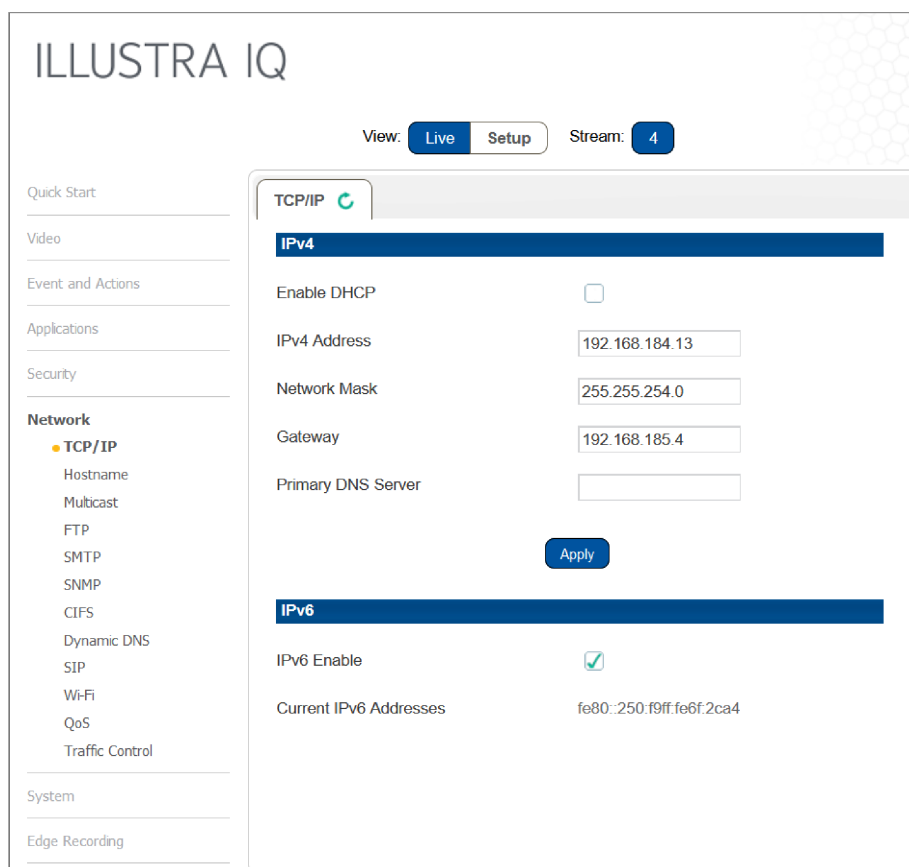
Figure 67 Network Menu
