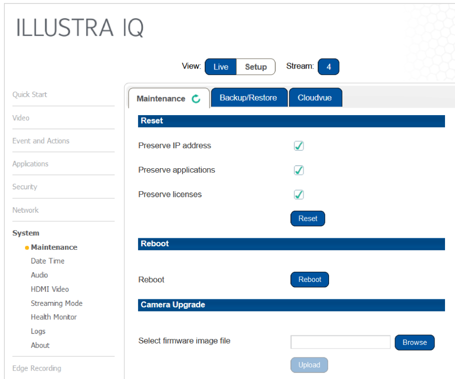
Figure 68 System Menu
